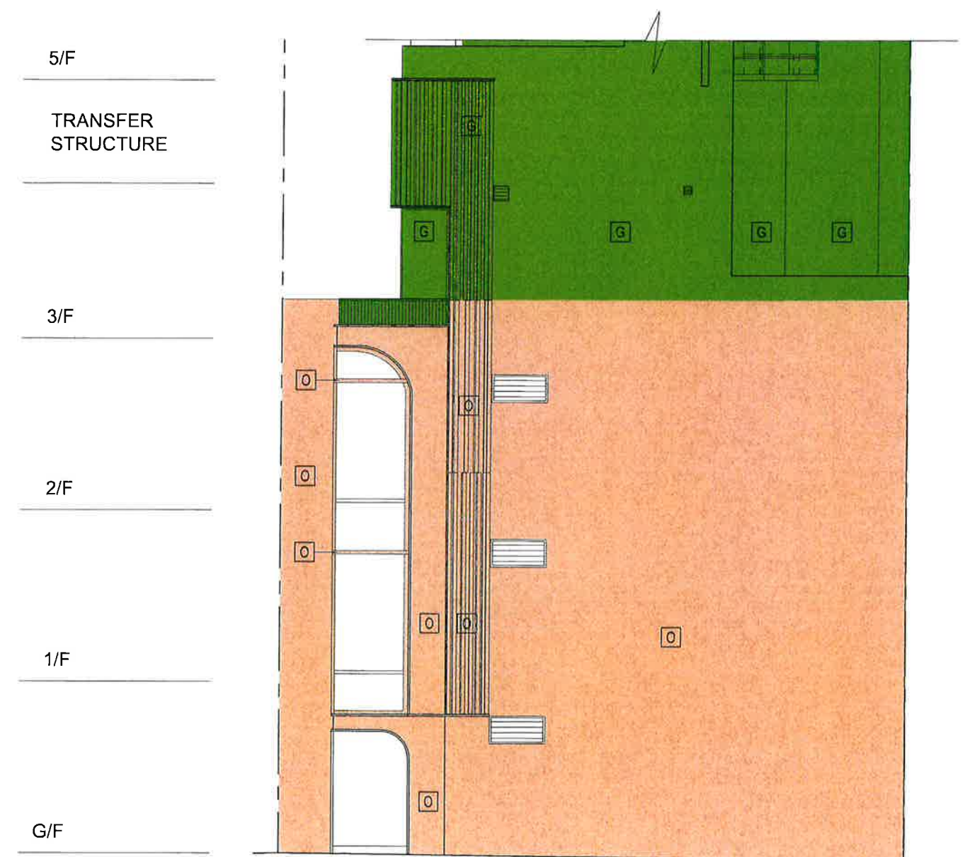
NORTH ELEVATION
