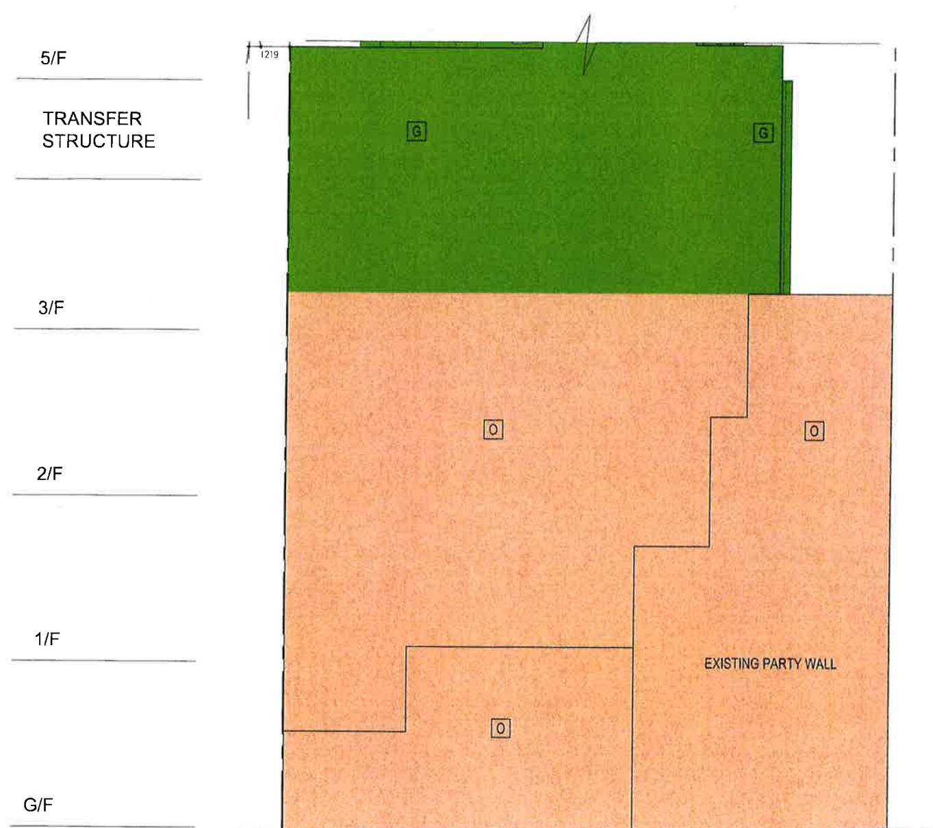
SOUTH ELEVATION
