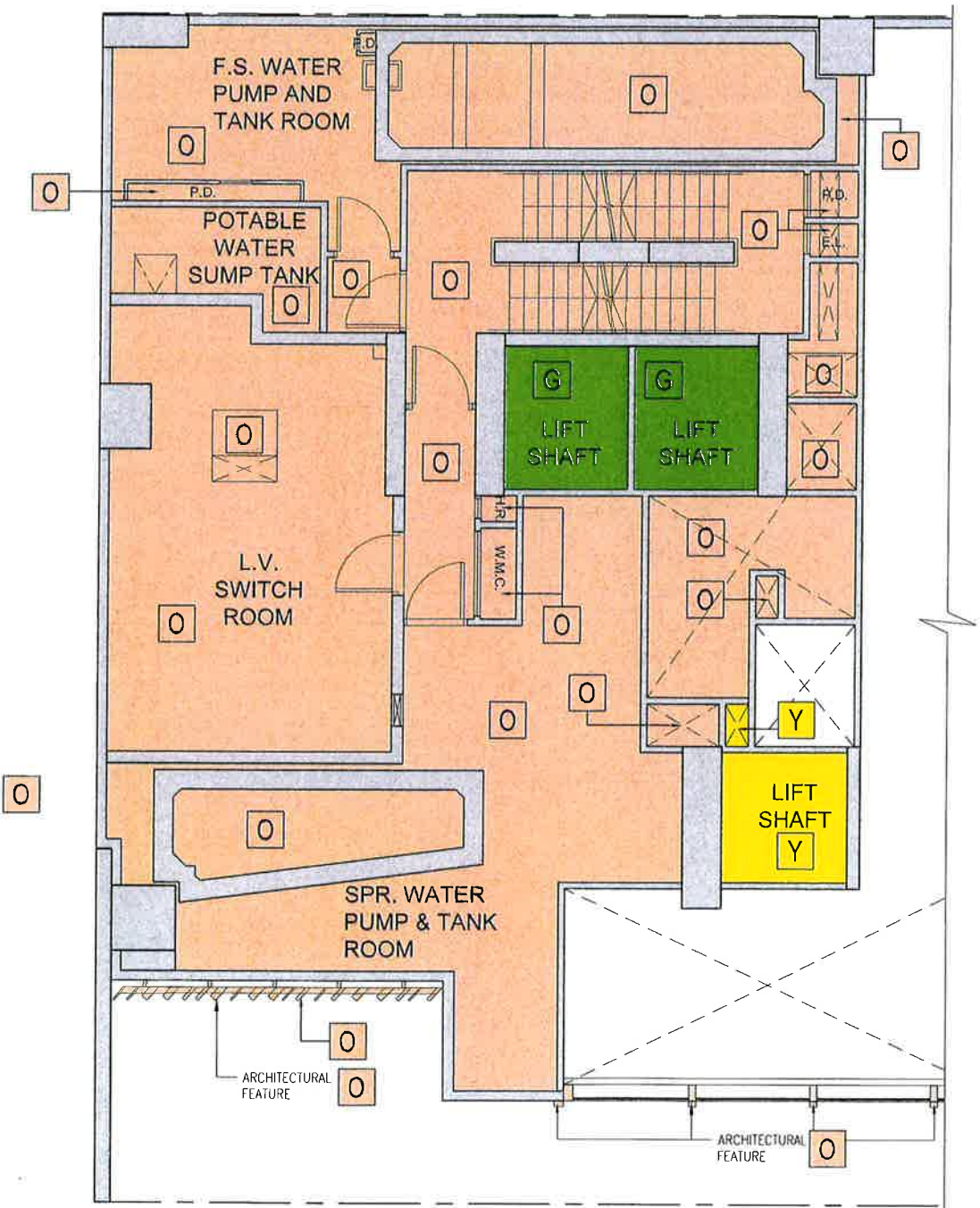
2/F FLOOR PART PLAN
